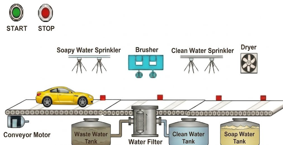
Fig. 4.1: Block Diagram of Automated Car Washing System with Water Recycling
